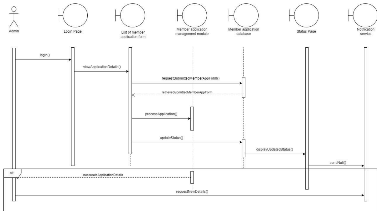
Figure 2.4.8.2: Sequence Diagram for Approve Membership Application
